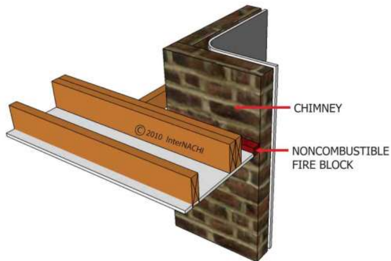
FIRE BLOCKING - CHIMNEY
