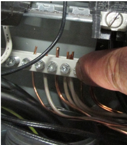
Three neutral conductors on one lug (only one allowed).
