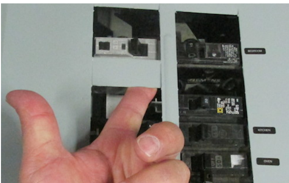
Breaker knockouts missing. Requires filler plates (blanks).
