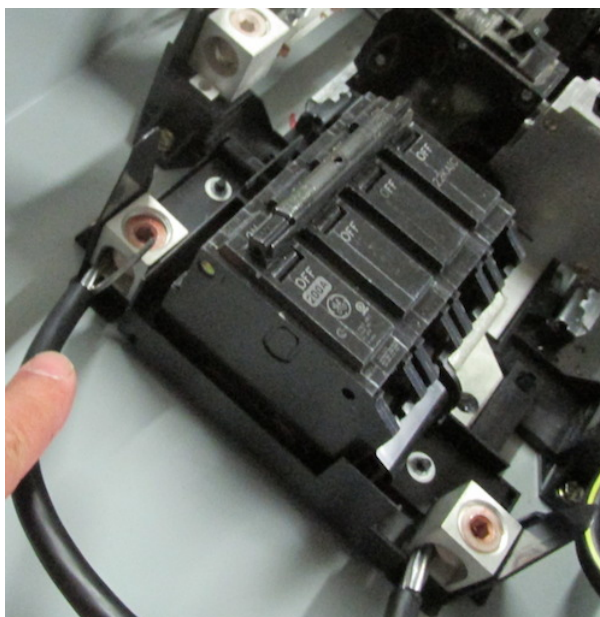
Not all strands are under set screw of lug.
