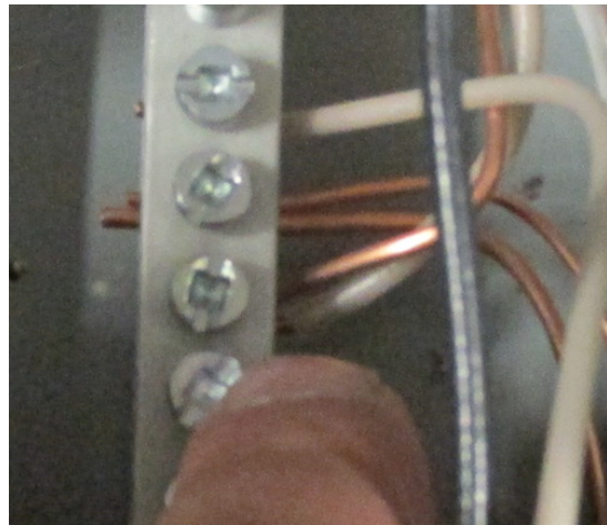
Ground and neutral conductor sharing same lug.
