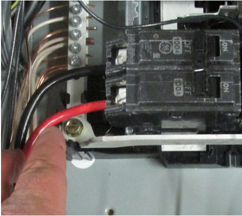
100 amp feeder breaker to subpanel protecting #6 conductor.
